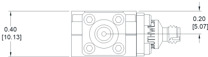
1.0 mm Connector View
