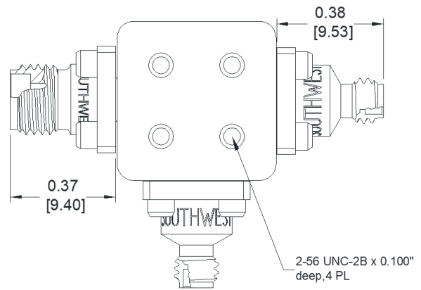
Bottomside View
