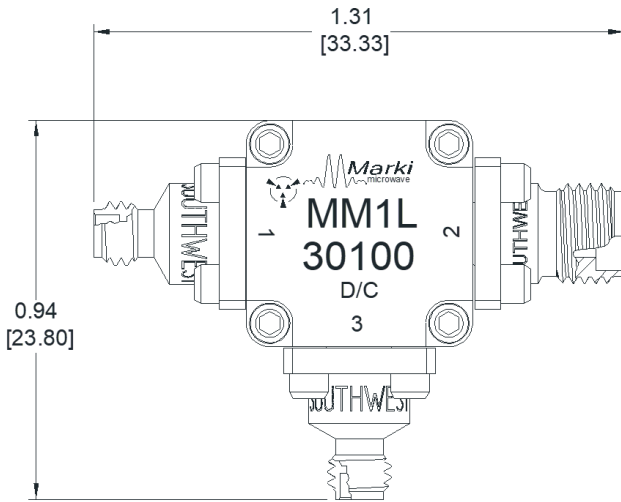
Topside View
