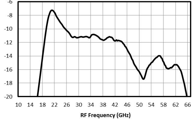
Vector Modulator Insertion Loss (dB) 6
