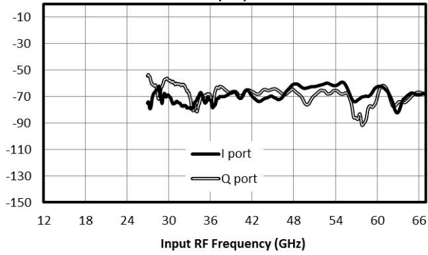
Spur Suppression, Downconversion, IF=14 GHz, LSLO, 5LOx-4RF (dBc) 7
