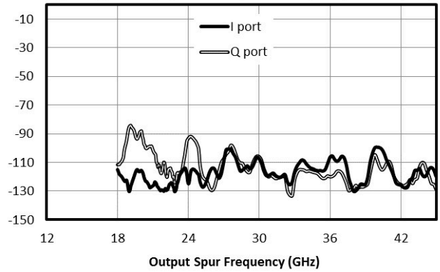
Spur Suppression, Downconversion, IF=91 MHz, LSLO, 2LOx2RF (dBc) 7
