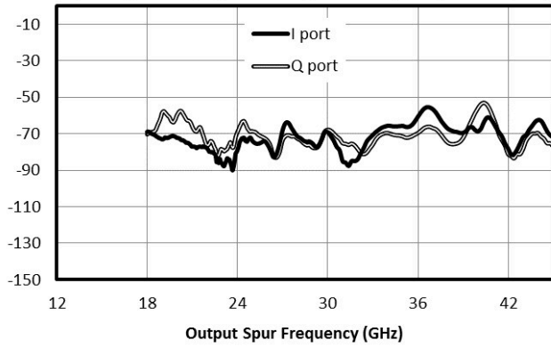
Spur Suppression, Upconversion, IF=91 MHz, LSLO, 1LOx5IF (dBc) 7
