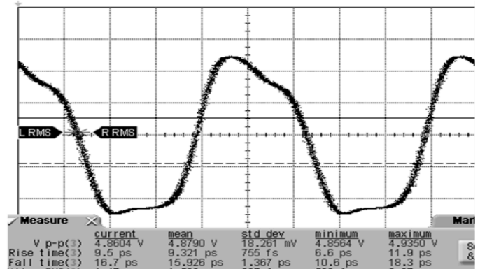
10 GHz, +5 dBm In, 5V/5V bias
