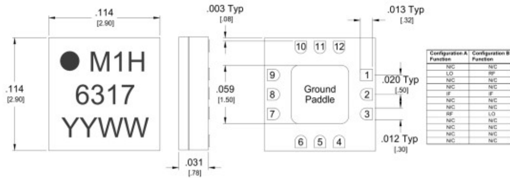
Outline Drawing – 3mm QFN package
