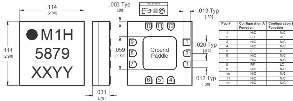
Outline Drawing – 3mm QFN package
