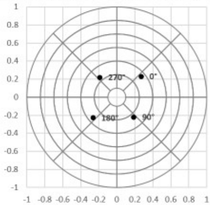
Vector Modulator Insertion Loss vs Phase: 20GHz (dB)
