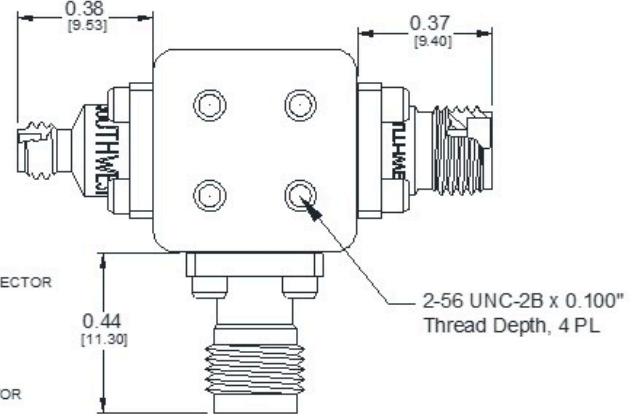
Bottomside View
