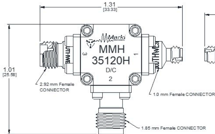
Topside View
