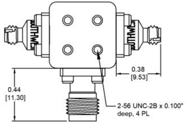
Bottomside View
