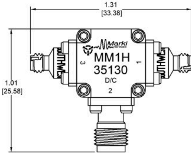
Topside View
