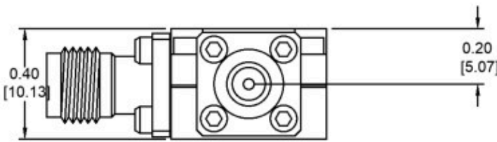
1.0 mm Connector View
